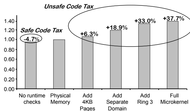
Figure 5. Normalized WebFiles execution time.
